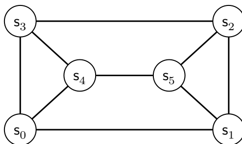
Figure 3 : Le graphe G
